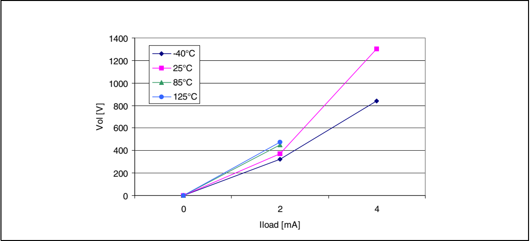
Figure 77. Typical V_{OL} at V_{DD} = 2.4\text{ V} (standard)
