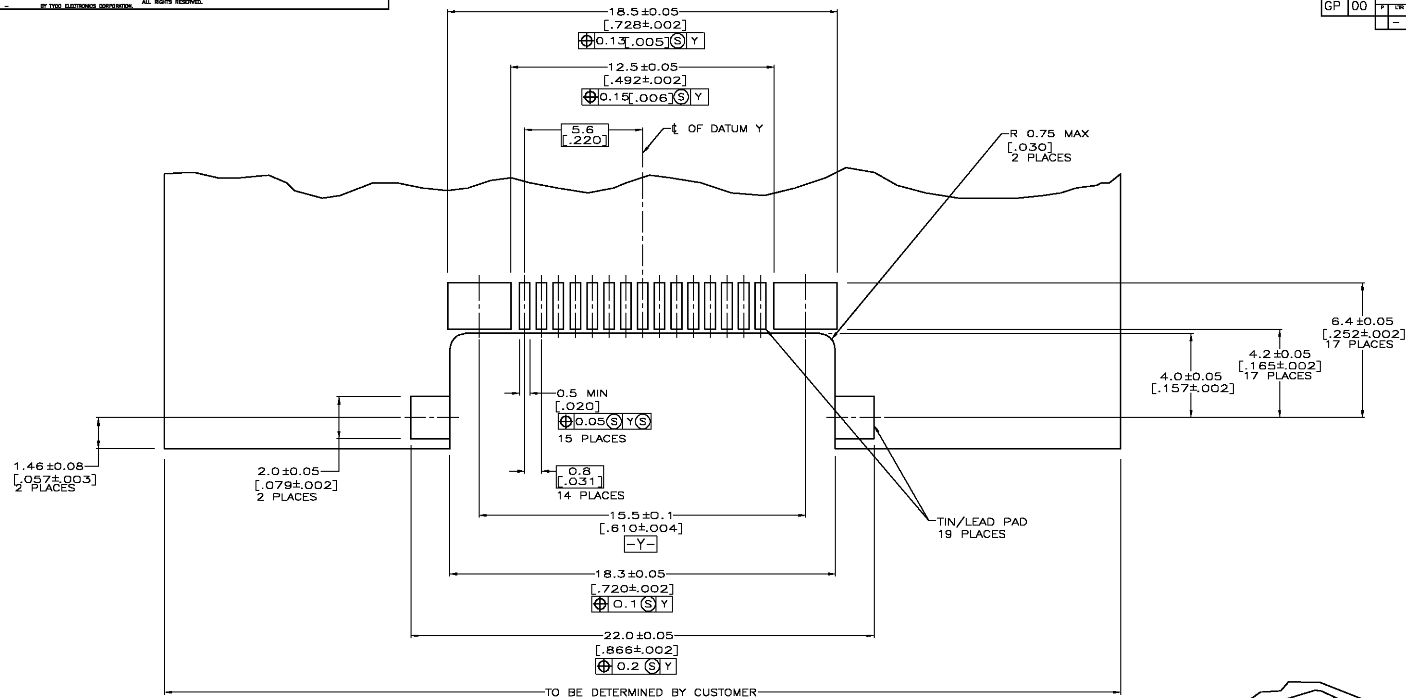
SUGGESTED PC BOARD MOUNTING DIMENSIONS
