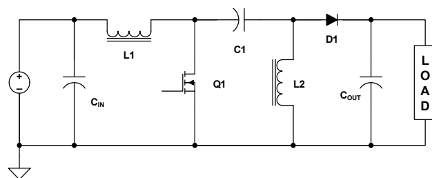
FIGURE 12. SEPIC TOPOLOGY
