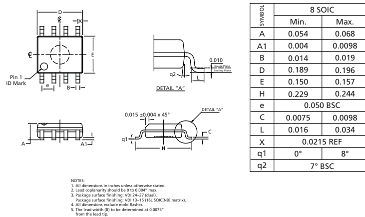
Figure 6-1: Package Dimensions
