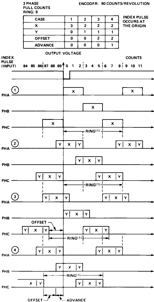
Figure 10. Commutator Configuration.
