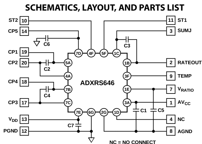
Figure 1. EVAL-ADXRS646Z Schematic
