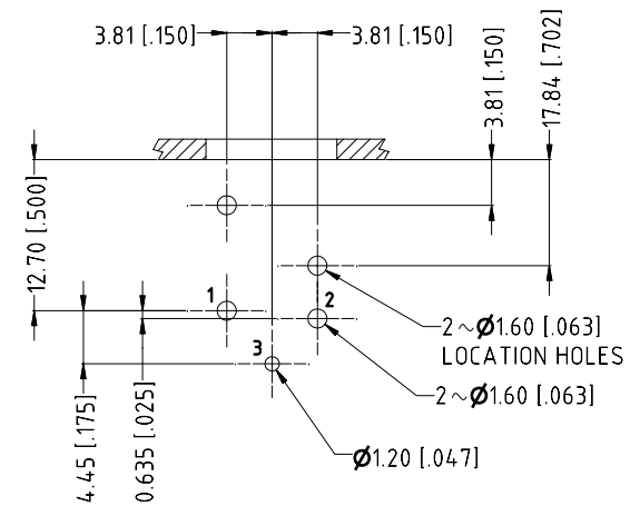
PCB LAYOUT COMPONENT SIDE TOLERANCE: ± 0.05mm [0.002"]
