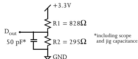
Figure B: Equivalent output load (AS4C1M16E5)
