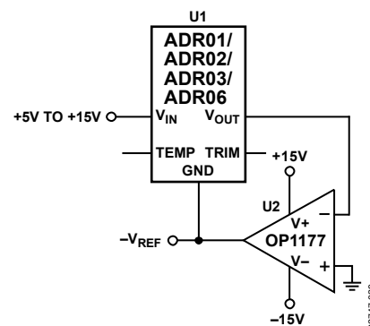
Figure 38. Negative Reference
