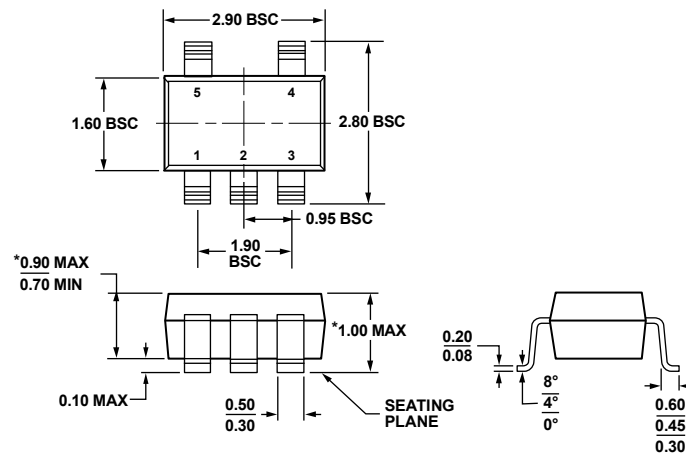
Figure 45. 5-Lead Thin Small Outline Transistor Package [TSOT] (UJ-5)
