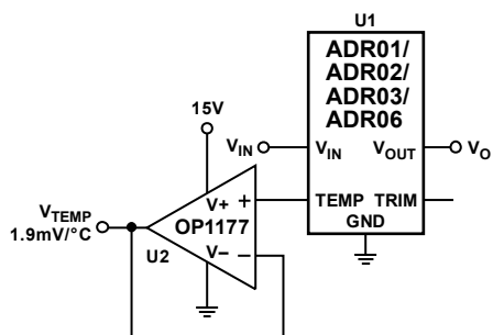
Figure 37. Temperature Monitoring
