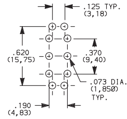
8261SH9_BE2 DPDT
