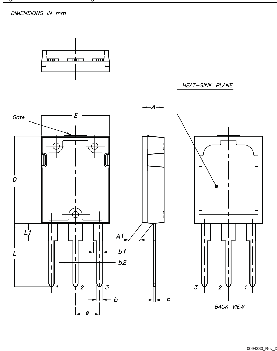
Figure 20. Max247 drawing
