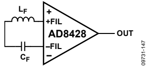
Figure 48. Notch Filter Example
