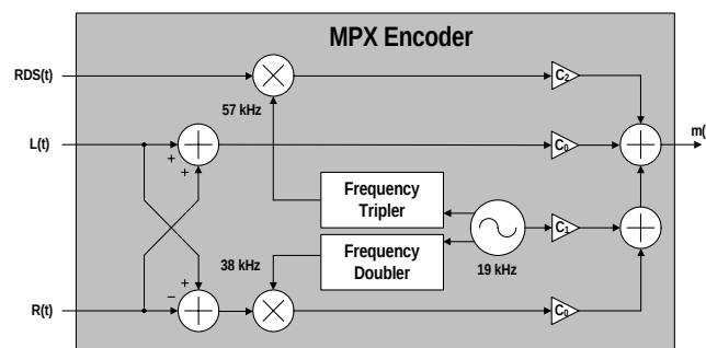
Figure 20. MPX Encoder
