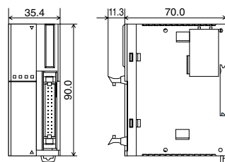
FC4A-D20K3, FC4A-D20S3
