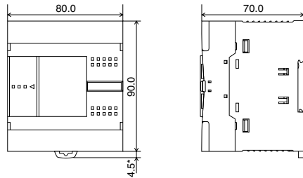
FC4A-D20K3, FC4A-D20S3
