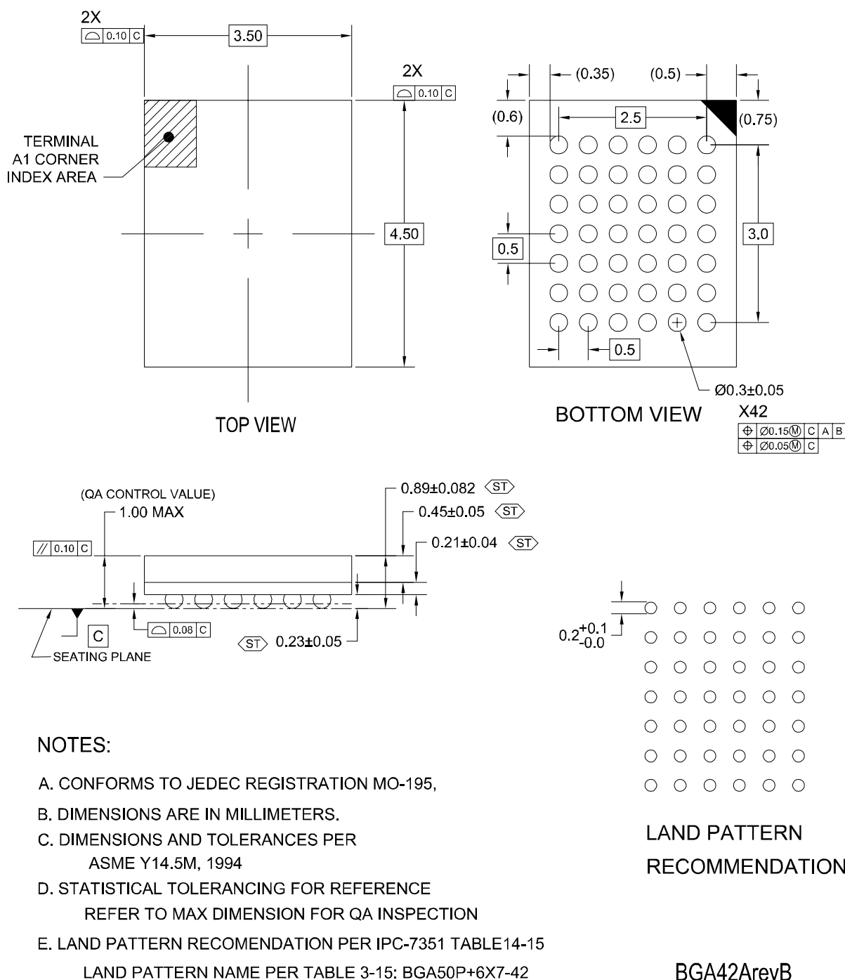
Figure 22. 42-Ball, Ball Grid Array (BGA) Package
