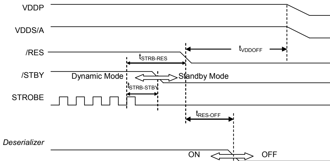
Figure 19. Power-Up Timing
