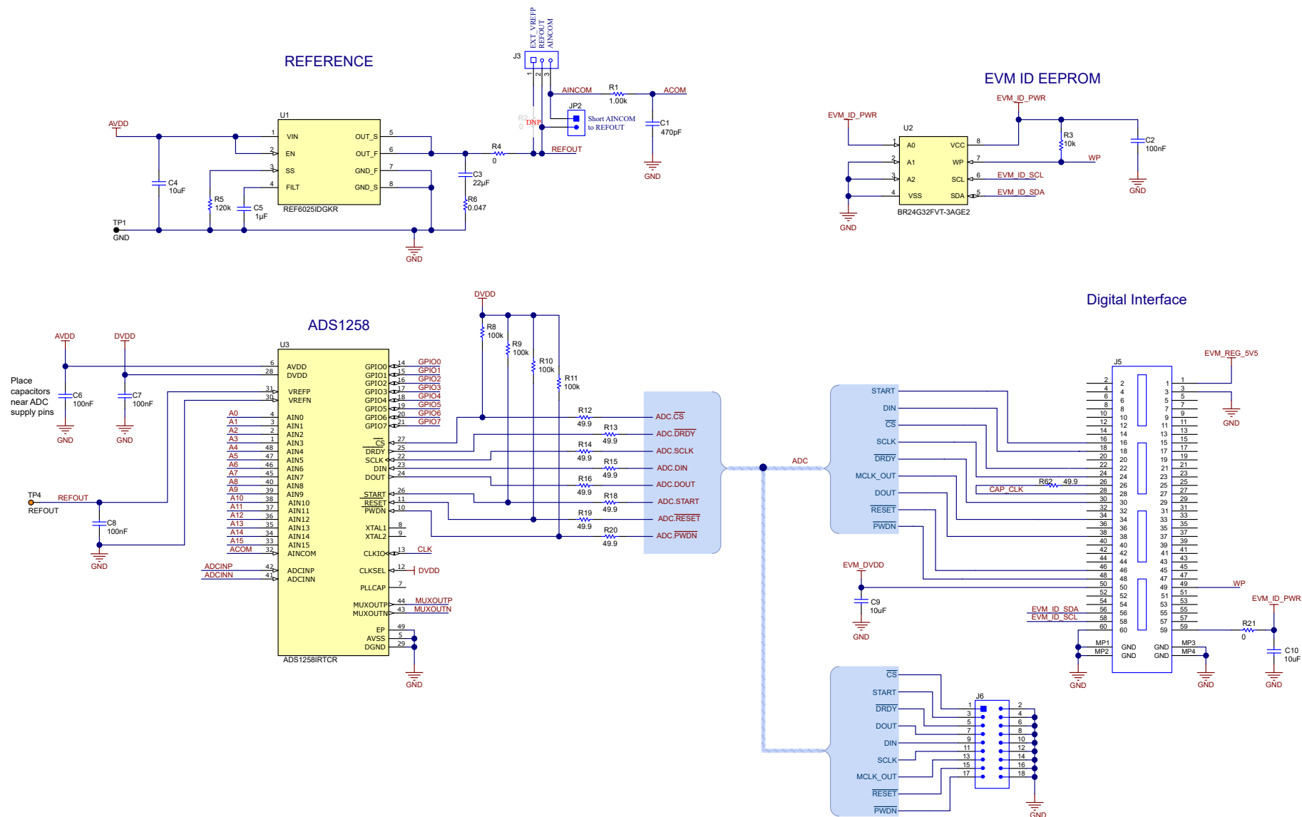
Figure 8-2. ADS1258EVM ADC, Voltage Reference, EEPROM, and Digital Interface Circuits
