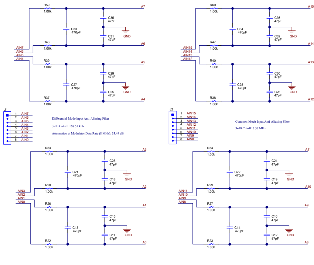
Figure 8-3. ADS1258EVM Analog Input, Multiplexer Loop, and GPIO Circuits
