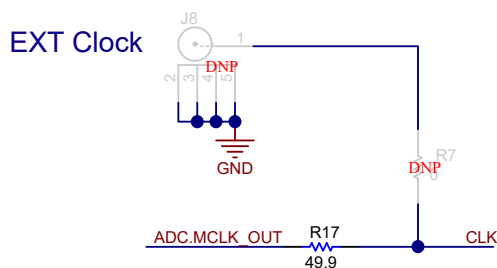
Figure 3-5. ADS1258EVM Clock Circuit
