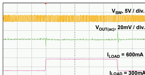
Figure 24. Fast Load Transient in CCM
