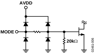
Figure 6. Equivalent MODE Input Circuit
