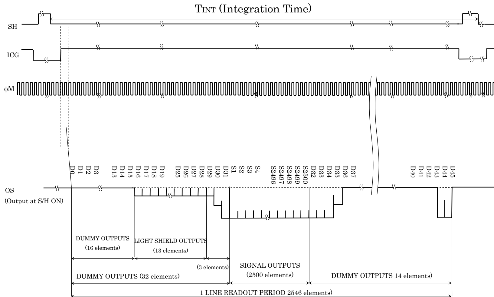
Timing Chart 1
