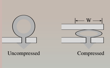
Electronic enclosure door shielding gasket
