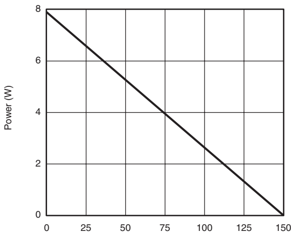
Power, Junction-to-Foot
