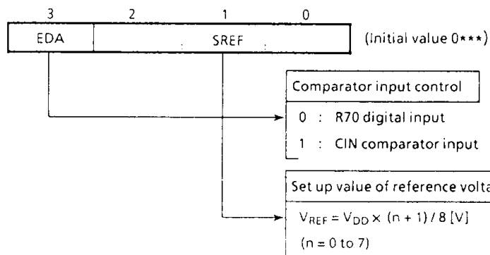
Figure 3-4. Command register
