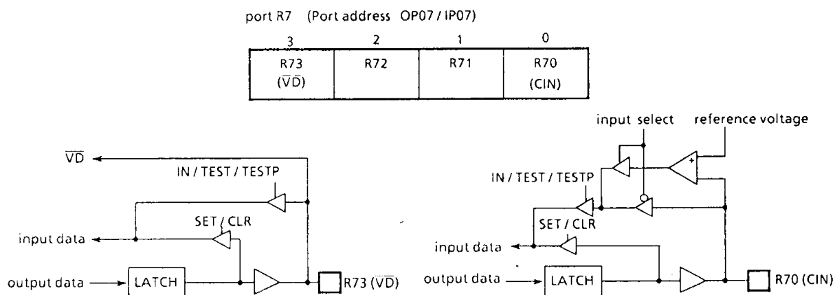
Figure 3-2. PORT R7
