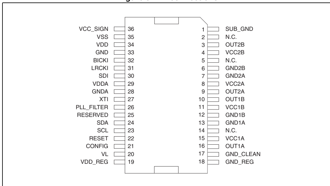
Figure 5. Pin connections
