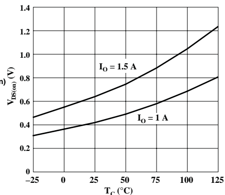
SLA7081MPR MOSFET V_{DS(on)} vs. Case Temperature
