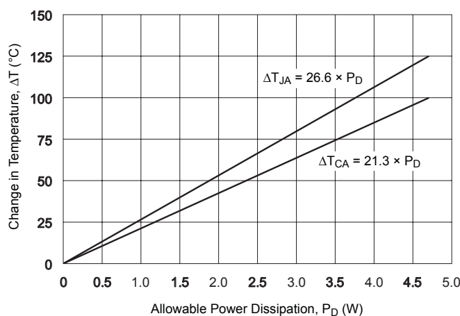
Figure 16. Power dissipation estimate for junction-to-ambient and case-to-ambient temperature change
