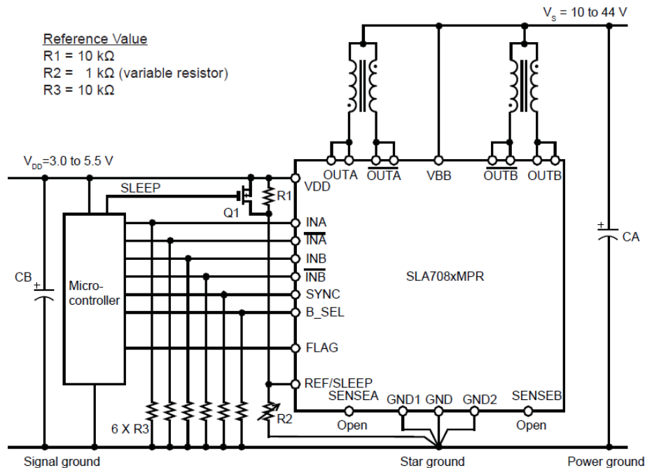
Figure 12. Typical application circuit using SLA7080MPR
