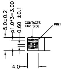
DETAIL A
