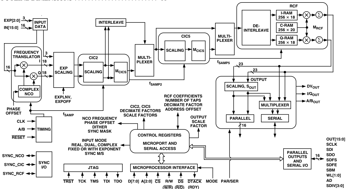
Figure 1. Block Diagram
