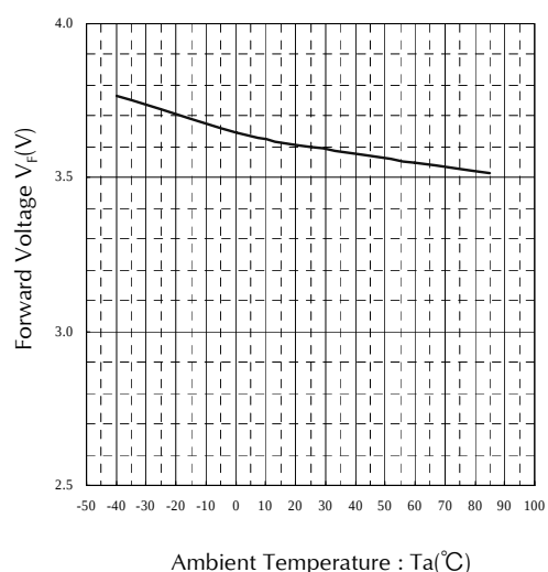
Ambient Temperature vs. Forward Voltage Condition : I_F = 300\text{mA}
