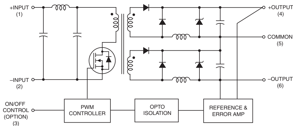
Figure 1. Simplified Schematic
