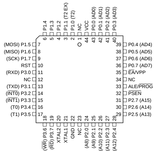
PLCC
