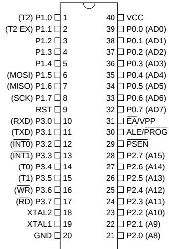
PDIP
