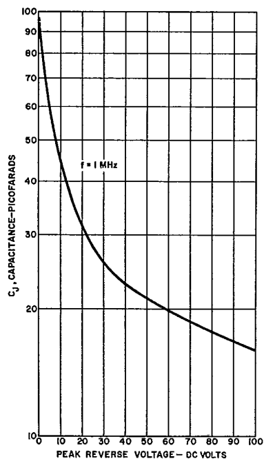
JUNCTION CAPACITANCE
