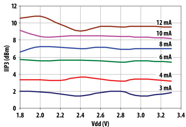
Figure 17. IIP3 vs. Vdd at 25°C
