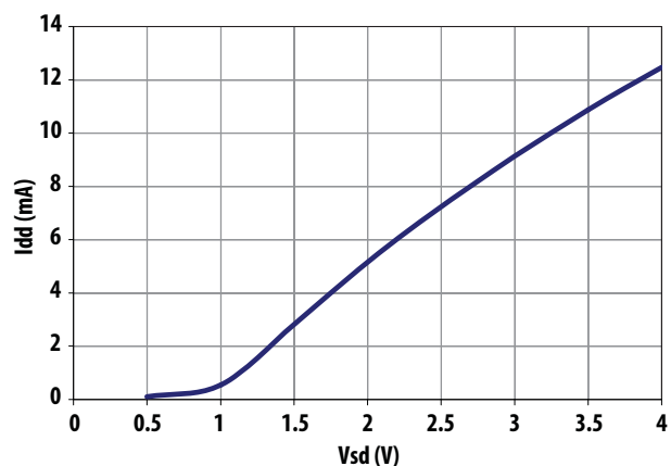
Figure 6. Idd vs Vsd for Vdd = 2.7V, Rbias = 8.2k Ohm
