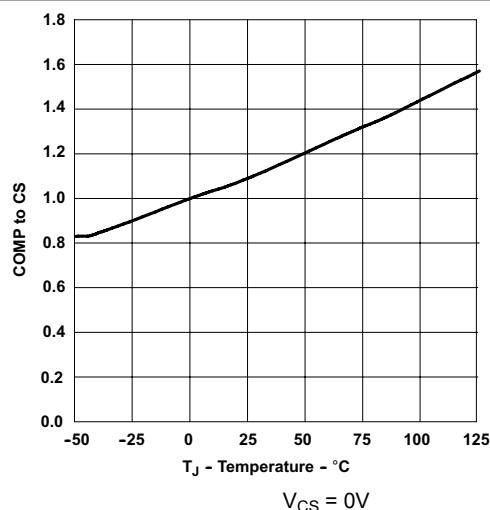
Figure 6-4. COMP to CS Offset Voltage vs Temperature
