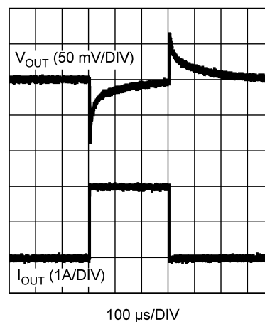
Figure 45. Transient Response I_{OUT} = 100\text{ mA} - 2A @ slewrate = 2A / \mu s
