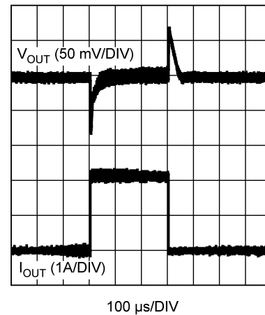
Figure 60. Transient Response I_{OUT} = 100\text{ mA} - 2\text{ A} @ slewrate = 2\text{ A} / \mu\text{s}
