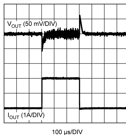
Figure 57. Transient Response I_{OUT} = 100\text{ mA} - 2A @ slewrate = 2A / \mu s
