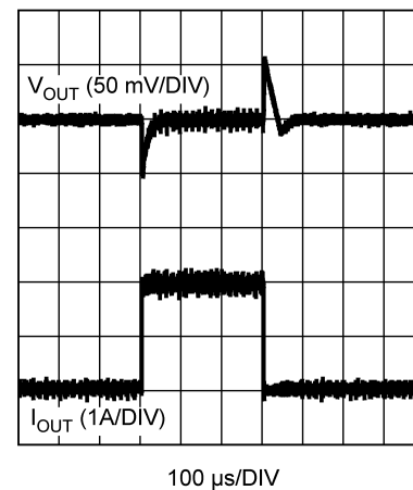
Figure 63. Transient Response I_{OUT} = 100\text{ mA} - 2\text{ A} @ slewrate = 2\text{ A} / \mu\text{s}
