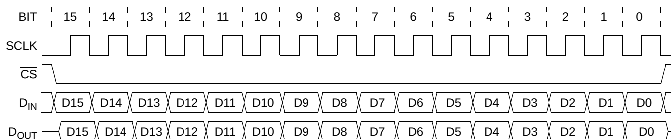
Figure 45. SPI Transfer Protocol
