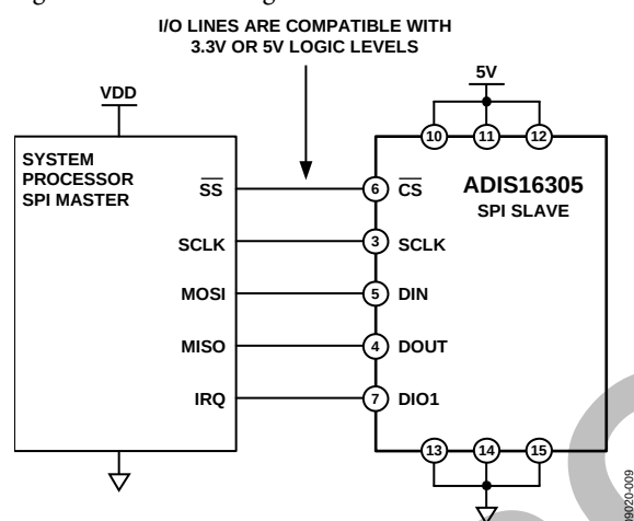
Figure 9. Electrical Connection Diagram
