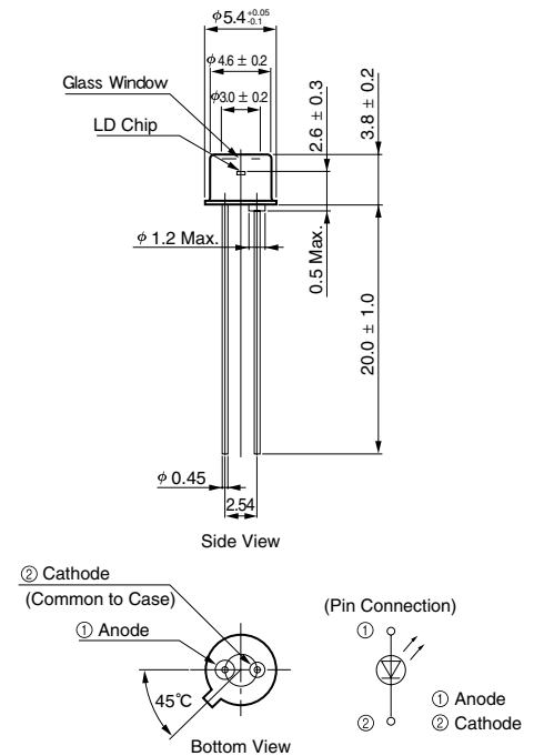
Figure 1: Dimensional Outline (Unit: mm)
