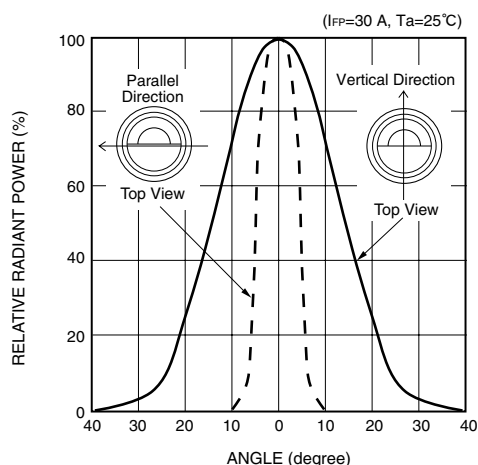
Figure 4: Typical Directivity
