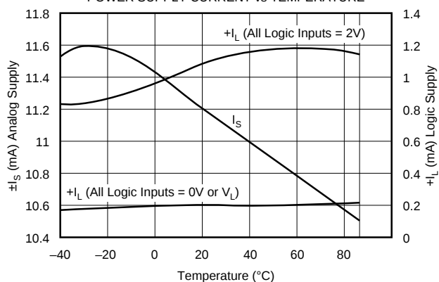
POWER SUPPLY CURRENT vs TEMPERATURE
