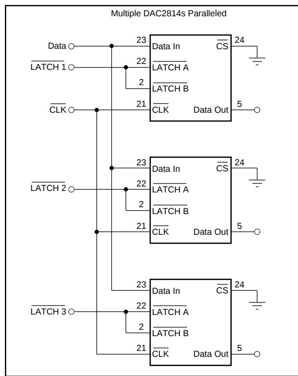
FIGURE 7. Parallel Bus Connection for Multiple DAC packages.
