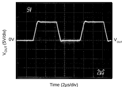
FULL-SCALE OUTPUT SWING UNIPOLAR (10V Step)
