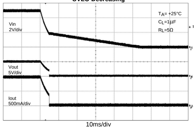
UVLO Decreasing
