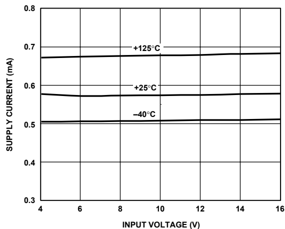
Figure 6. ADR435 Supply Current vs. Input Voltage
