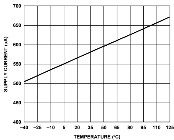
Figure 7. ADR435 Supply Current vs. Temperature
