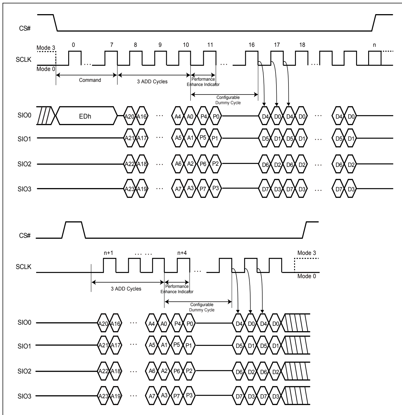
Figure 61. 4 x I/O DT Read Performance Enhance Mode Sequence (SPI Mode)
