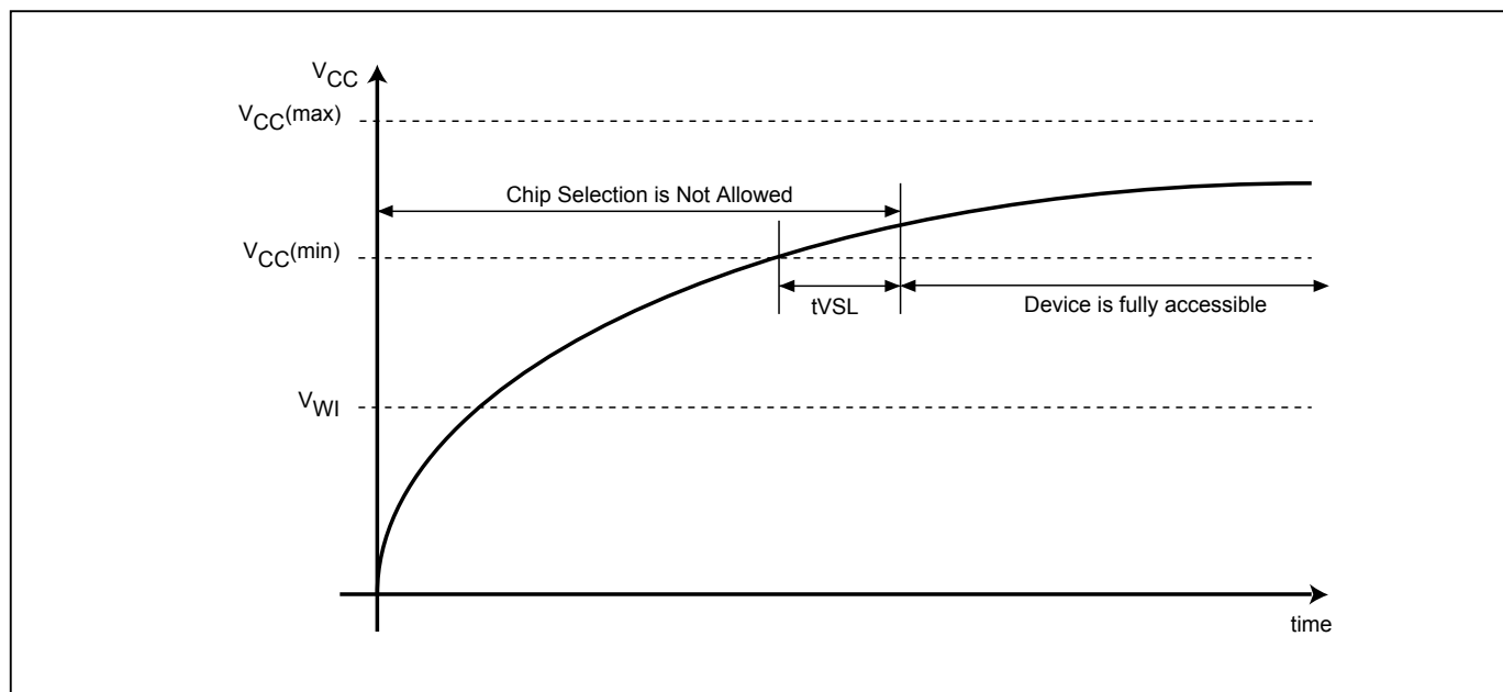
Figure 111. Power-up Timing
