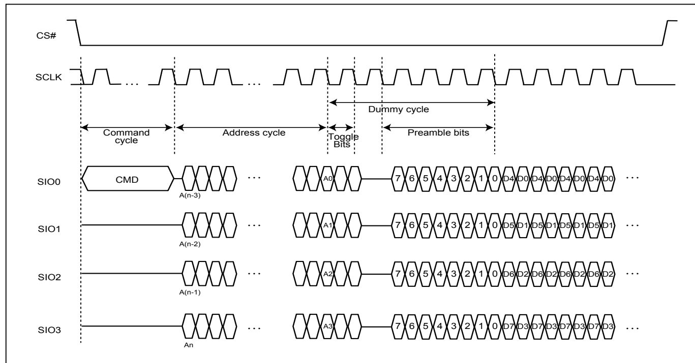
Figure 47. DTR4IO (6DC)
