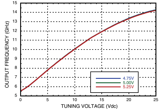
Frequency vs. Tuning Voltage, T = +25^{\circ}C
