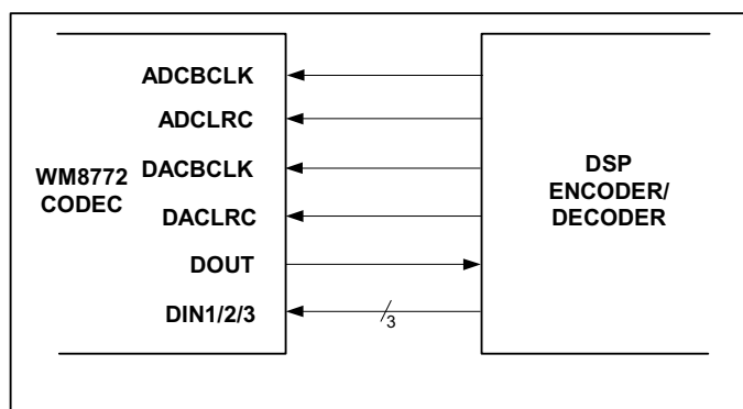
Figure 41 Slave Mode
