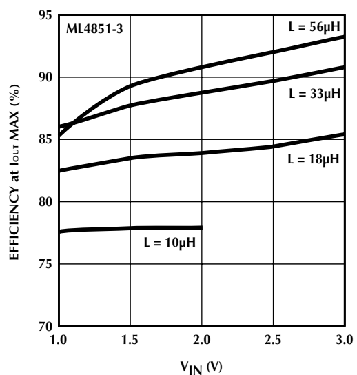
Figure 5. Typical Efficiency as a Function of V_{IN}
