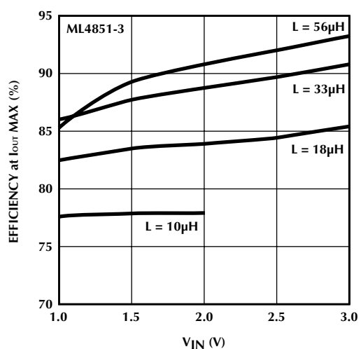
Figure 5. Typical Efficiency as a Function of V_{IN}
