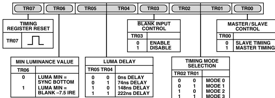
Figure 66. Timing Register 0
