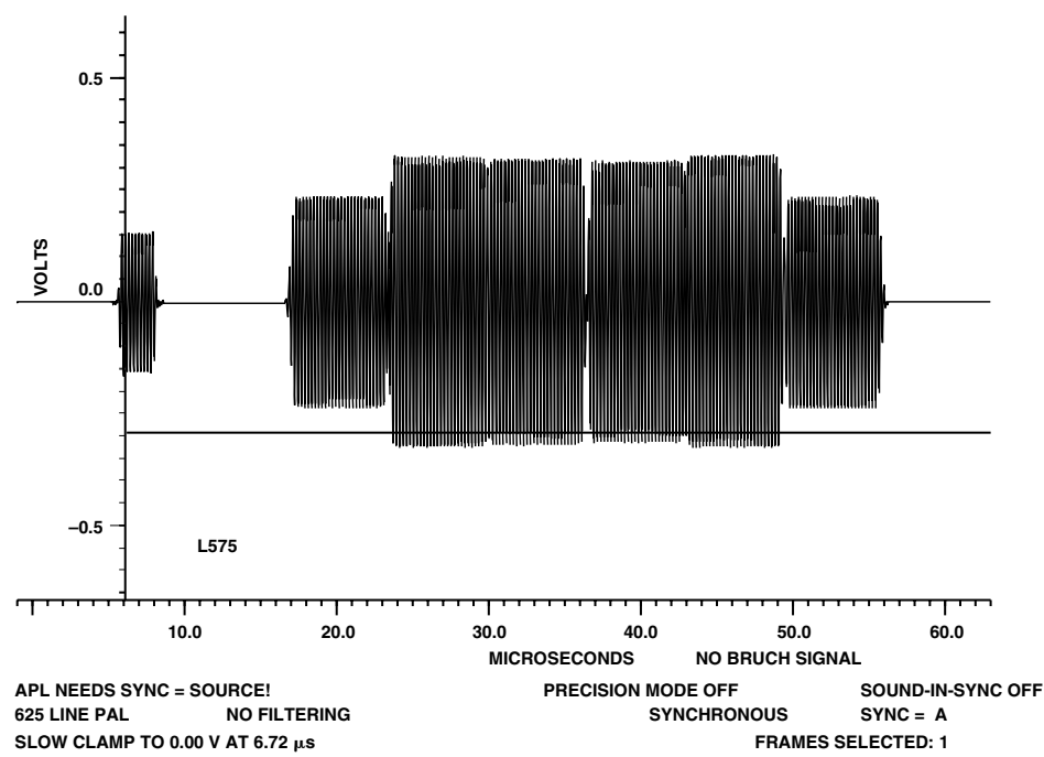
Figure 129. 100%/75% PAL Color Bars Chrominance
