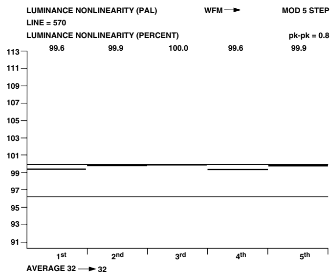
Figure 138. PAL Luminance Nonlinearity
