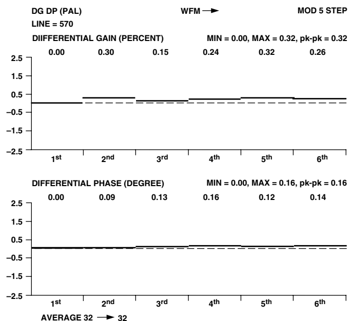
Figure 137. PAL DG DP Measurement
