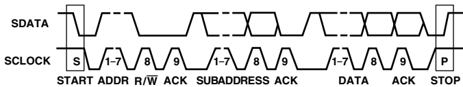
Figure 52. Bus Data Transfer
