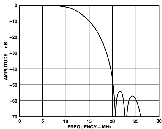
Figure 33. Plot of the Interpolation Filter for the CrCb Data
