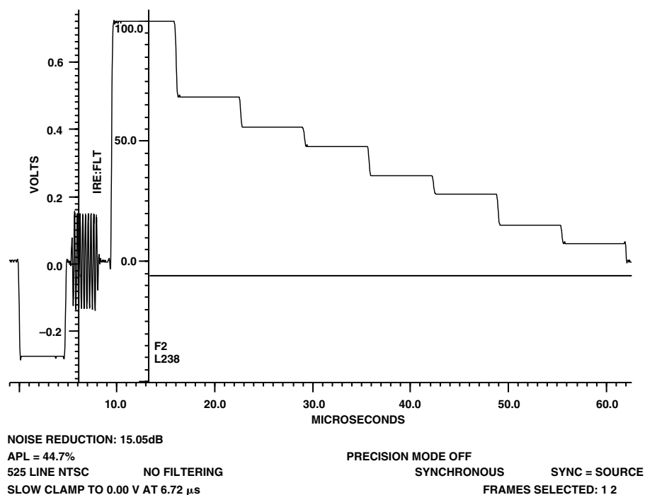
Figure 131. 100%/75% NTSC Color Bars Luminance
