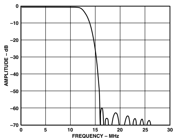
Figure 32. Plot of the Interpolation Filter for the Y Data
