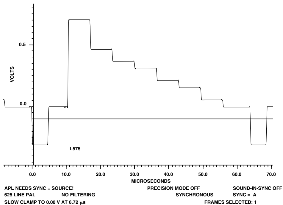
Figure 128. 100%/75% PAL Color Bars Luminance
