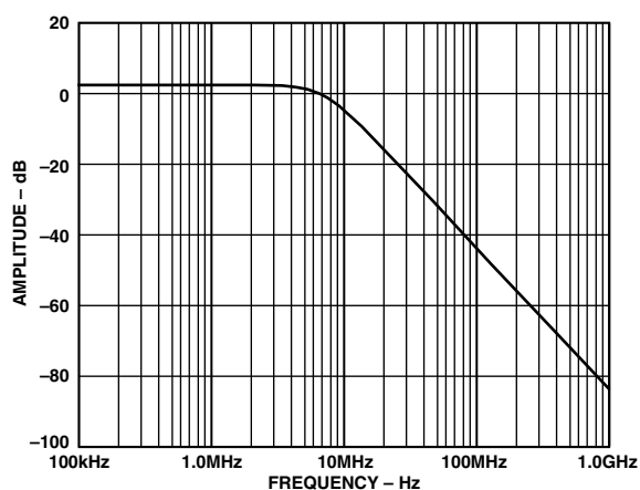
Figure 103. Output Filter Plot for 4× Oversampling Filter
