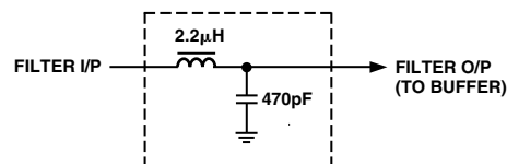
Figure 102. Output Filter for 4× Oversampling Mode
