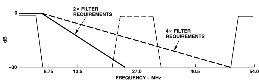
Figure 104. Output Filter Requirements in 4× Oversampling Mode
