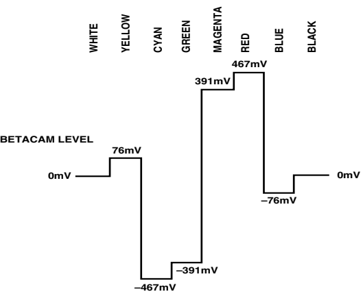
Figure 125. NTSC 100% Color Bars with Pedestal V
