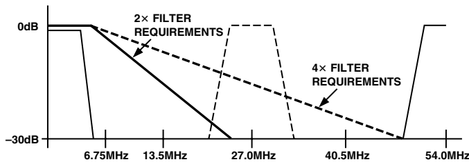
Figure 8. Output Filter Requirements in 2× and 4× Oversampling Mode
