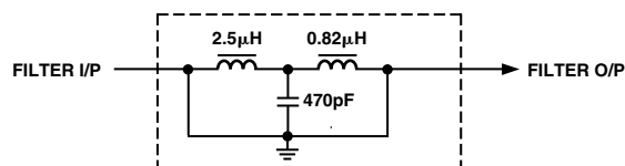
Figure 100. Output Filter for 2× Oversampling Mode
