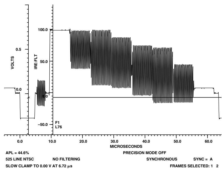
Figure 130. 100%/75% NTSC Color Bars
