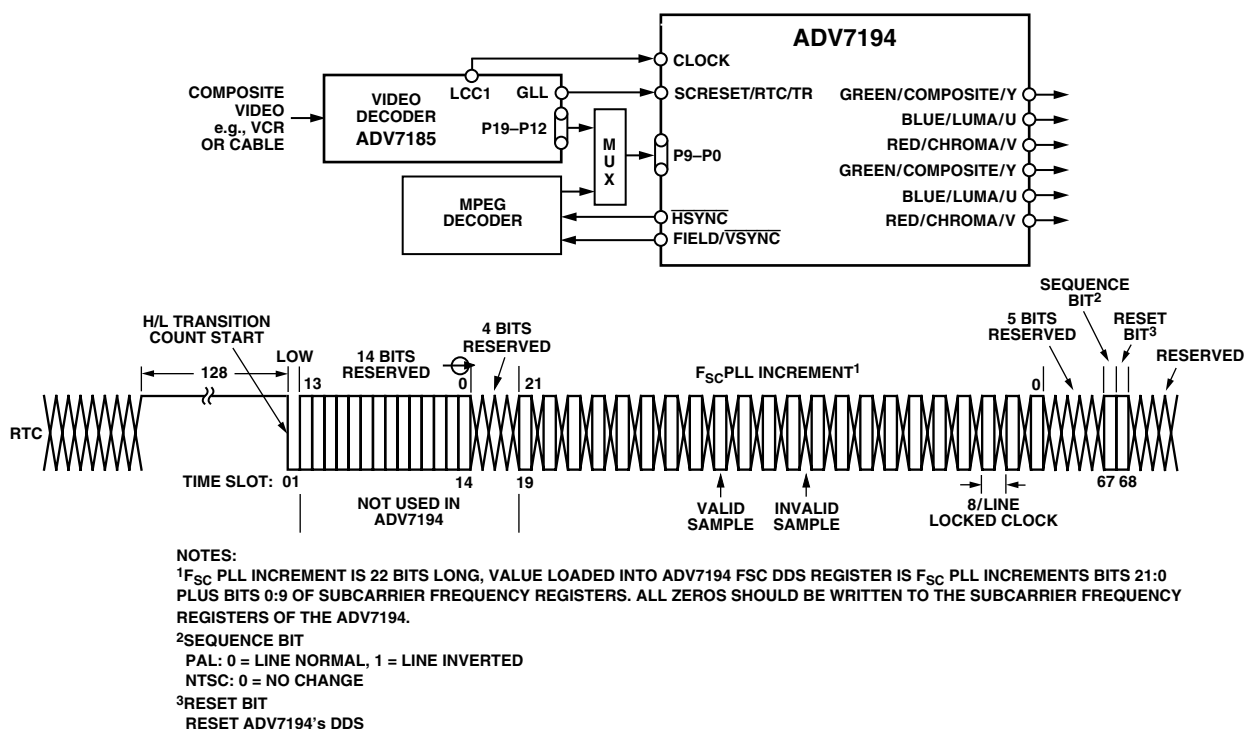
Figure 37. RTC Timing and Connections
