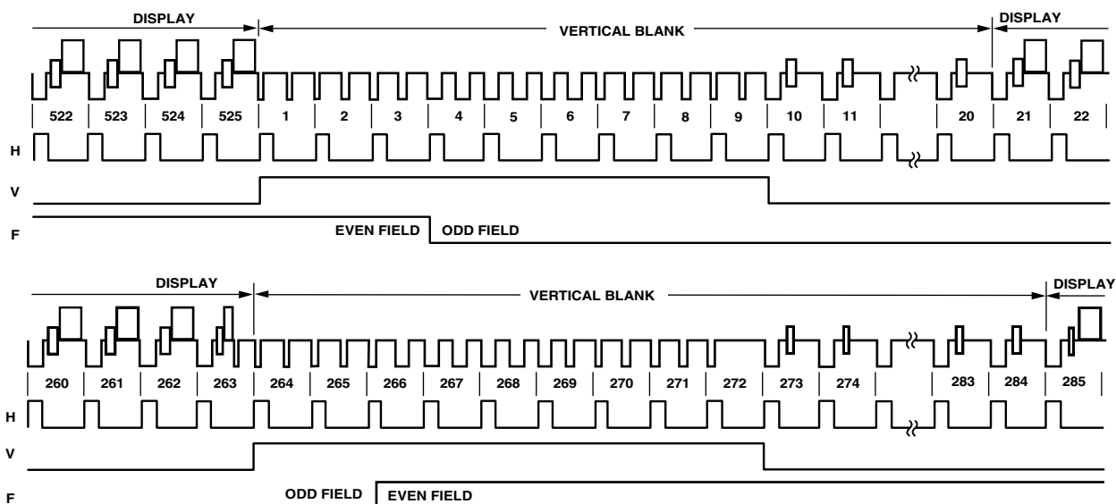
Figure 39. Timing Mode 0, NTSC Master Mode
