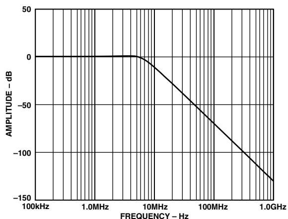
Figure 101. Output Filter Plot for 2× Oversampling Filter
