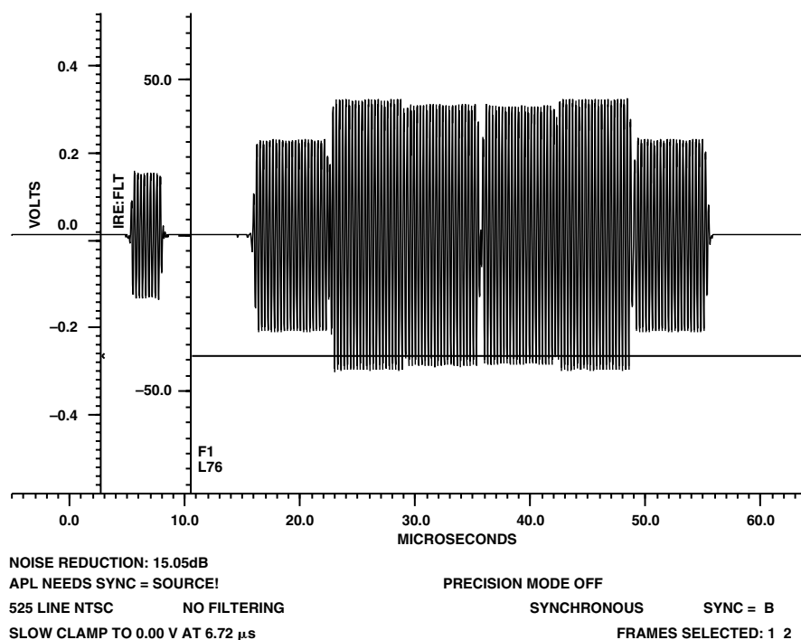
Figure 132. NTSC Color Bars Chrominance
