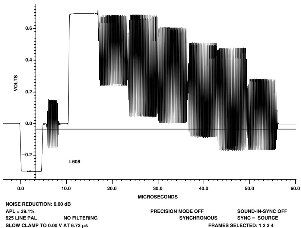
Figure 127. 100%/75% PAL Color Bars
