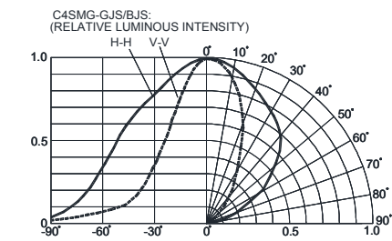
FIG.6 BLUE&GREEN FAR FIELD PATTERN
