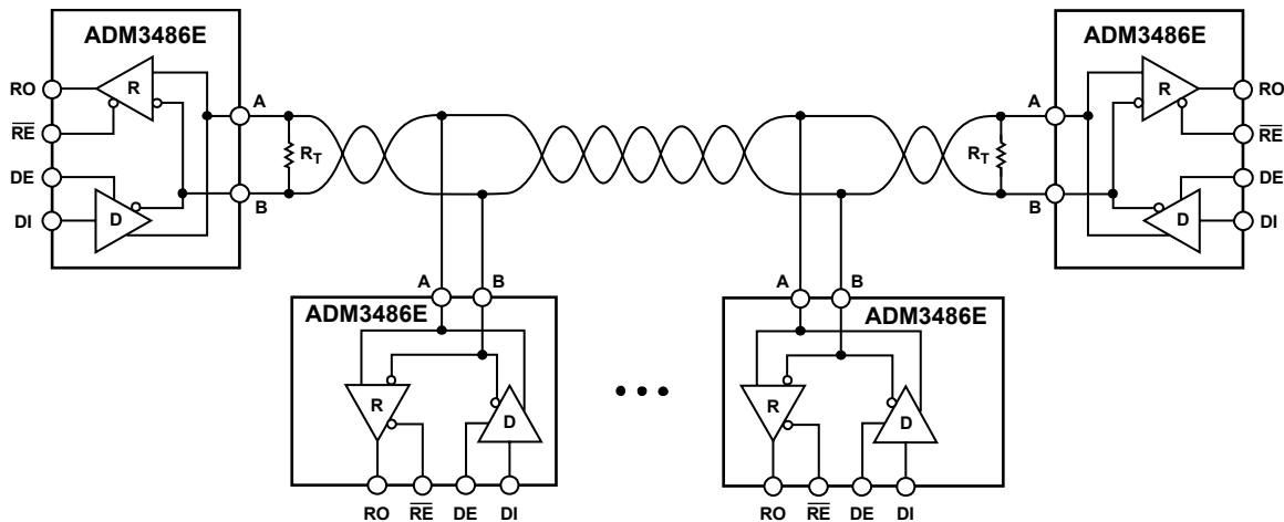
Figure 29. ADM3486E Typical Half-Duplex RS-485 Network
