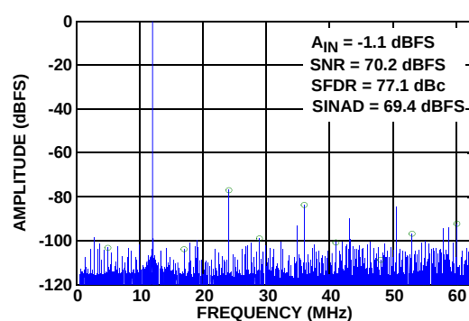
FIGURE 18. SINGLE-TONE SPECTRUM @ 363MHz
