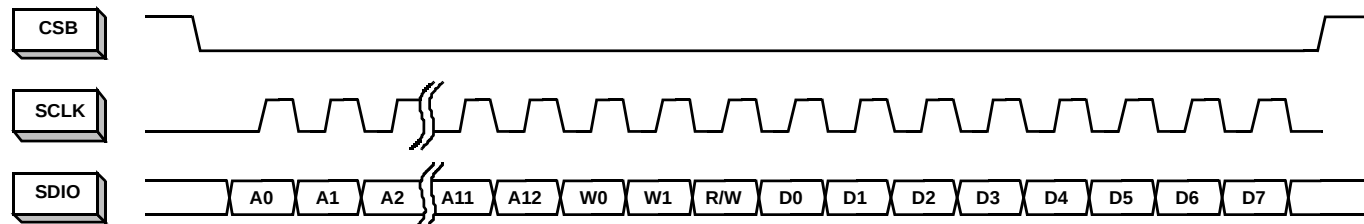
FIGURE 39. LSB-FIRST ADDRESSING
