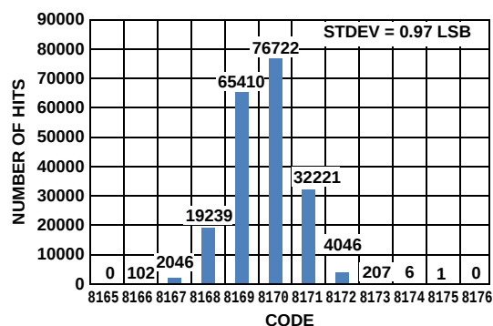
FIGURE 15. NOISE HISTOGRAM
