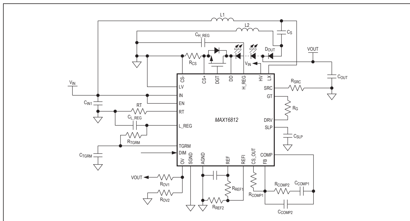
Figure 15. SEPIC Configuration
