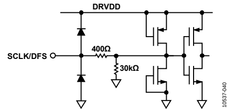
Figure 47. Equivalent SCLK/DFS Input Circuit
