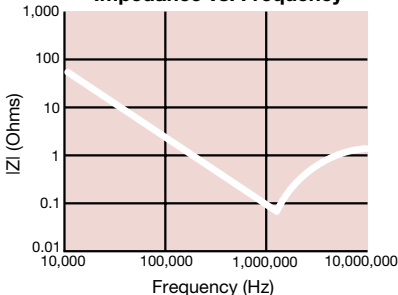
0.22 μF - 0805 Impedance vs. Frequency
