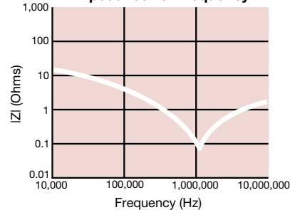
1 μF - 1206 Impedance vs. Frequency
